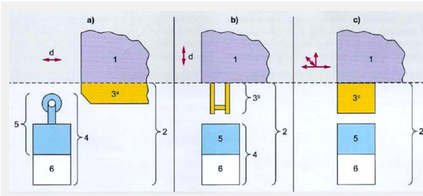
Fig 2: Principles of Type 1, Type 2, Type 3 and Type 4 interlocking devices.
