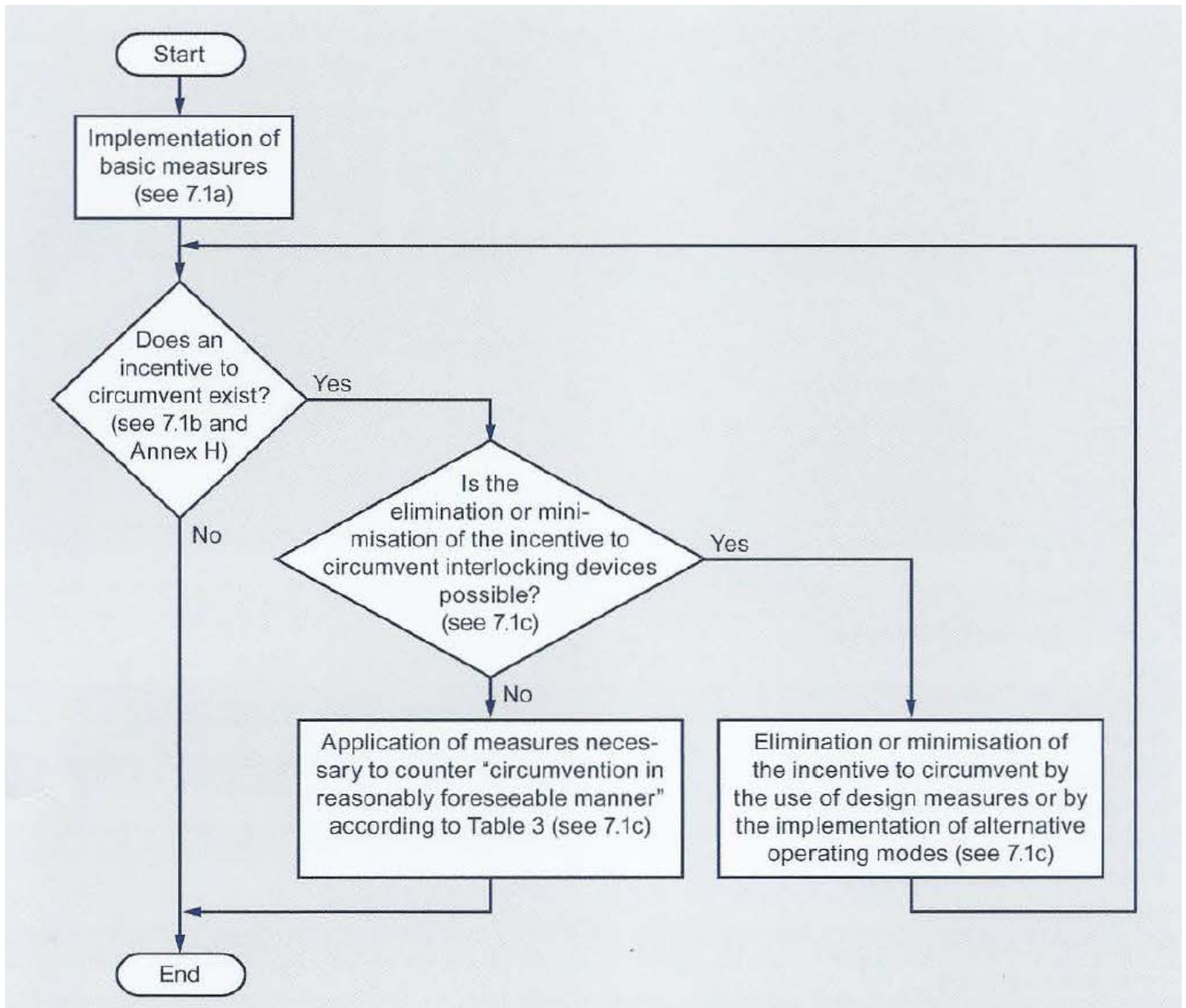
Fig 12: Method to determine the possible incentive to tamper with interlocking devices and the requisite measures to be taken by the manufacturer
