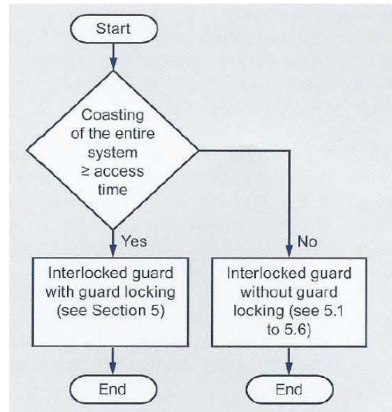
Fig 11: Determination of the need for a locking interlock device
